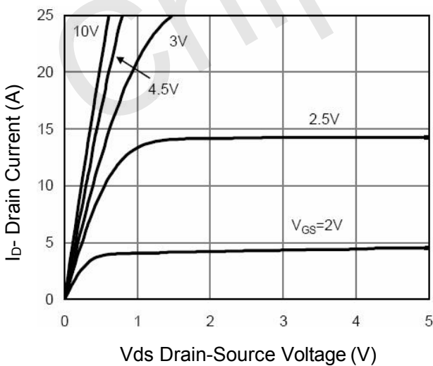
Figure 5 Output Characteristics
