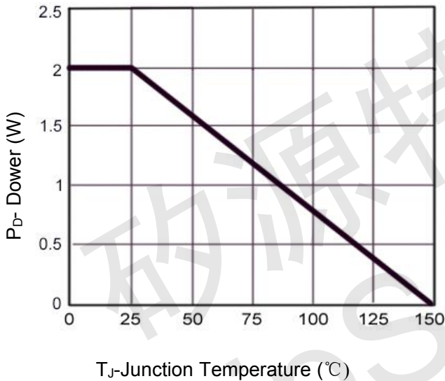
Figure 3 Power De-rating
