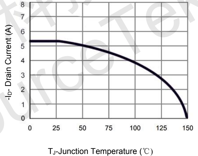
Figure 4 Drain Current
