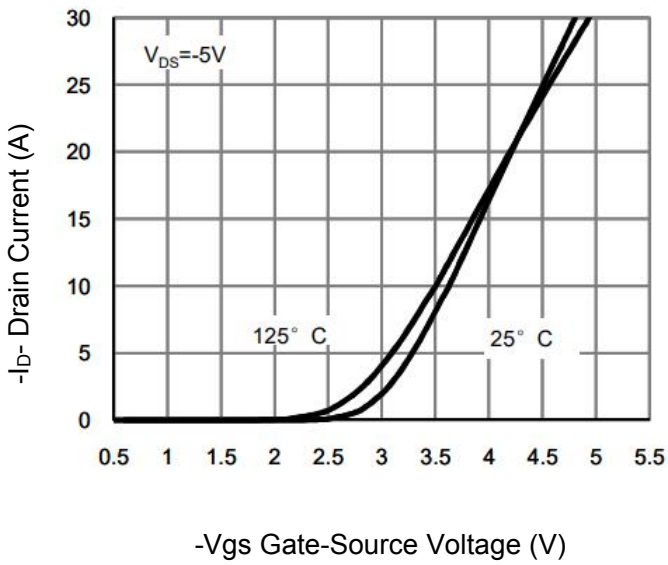
Figure 7 Transfer Characteristics
