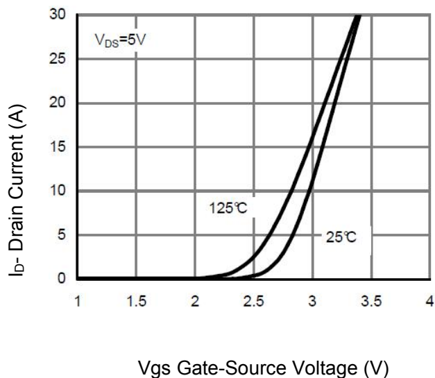
Figure 7 Transfer Characteristics
