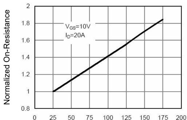
Figure 8 Rdson vs Junction Temperature
