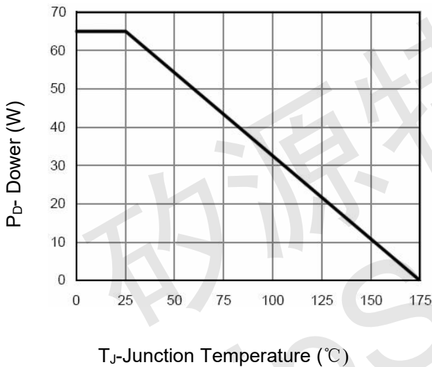
Figure 3 Power De-rating
