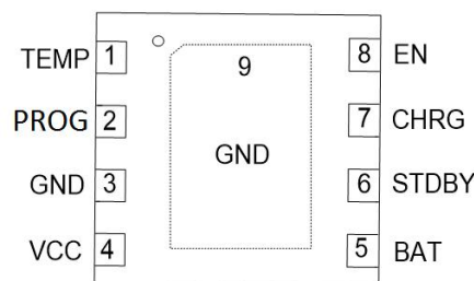
DFN2*2-8L
