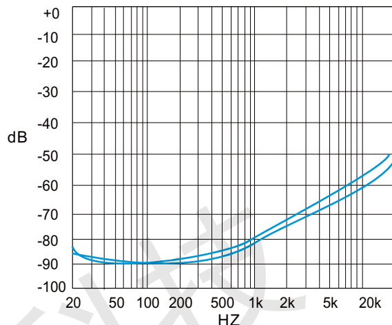
PSRR vs. Freq SE mode, 3V, 32Ohm, 200mVpp Input untermiated
