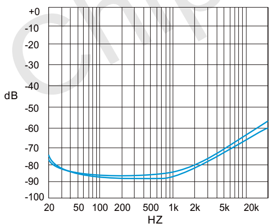
PSRR vs. Freq SE mode, 6V, 320hm, 200mVpp Input terminated
