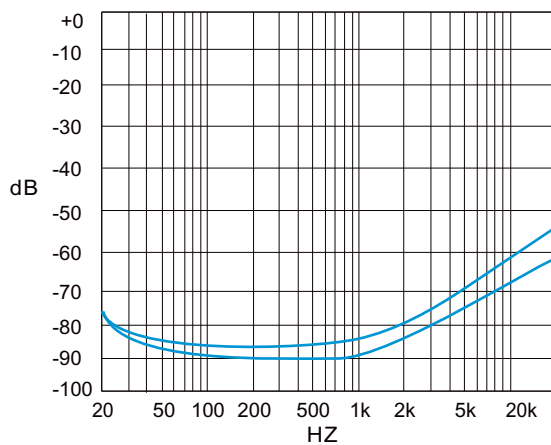
PSRR vs. Freq SE mode, 3V, 320hm, 200mVpp Input terminated
