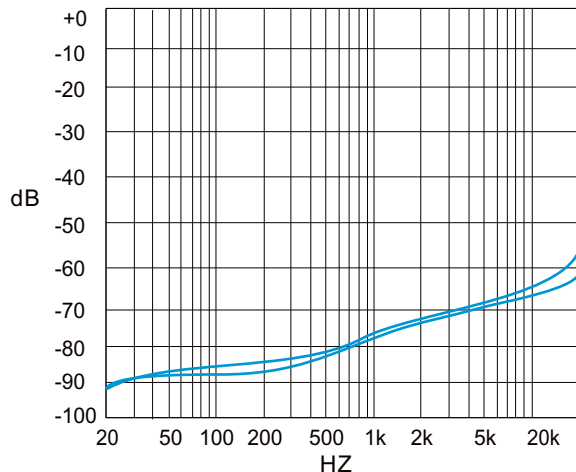
PSRR vs. Freq SE mode, 6V, 32Ohm, 200mVpp Input untermiated
