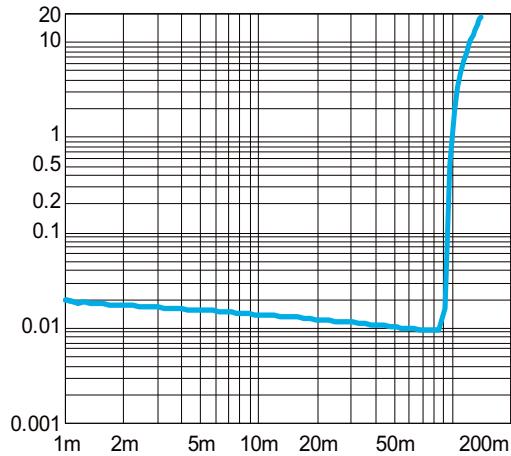
THD+N vs. Output Power SE mode, 5V, 320hm, f=1 kHz
