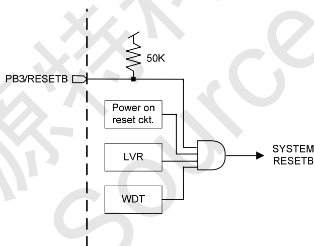
Figure 4 Reset structure
