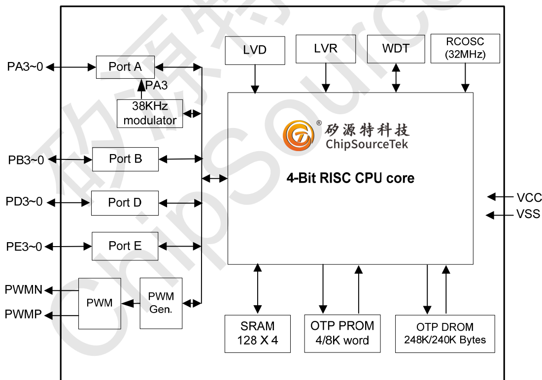
Figure 2. Block diagram
