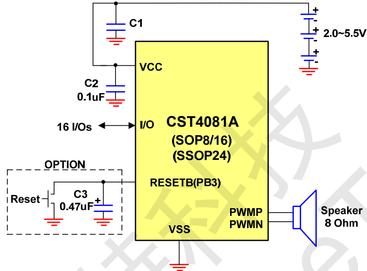
Figure 5 PWM Applications circuit
