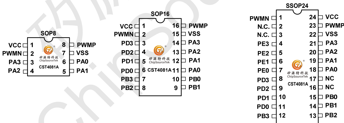
Figure1. Package definition
