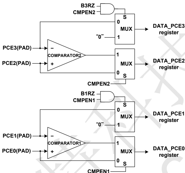
Figure 11. Port PCE mode 2 block diagram
