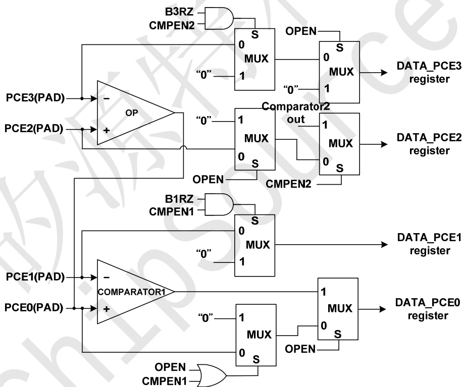
Figure 12. Port PCE mode 3 block diagram
