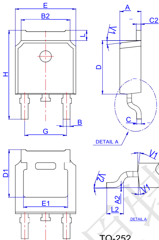
TO-252
