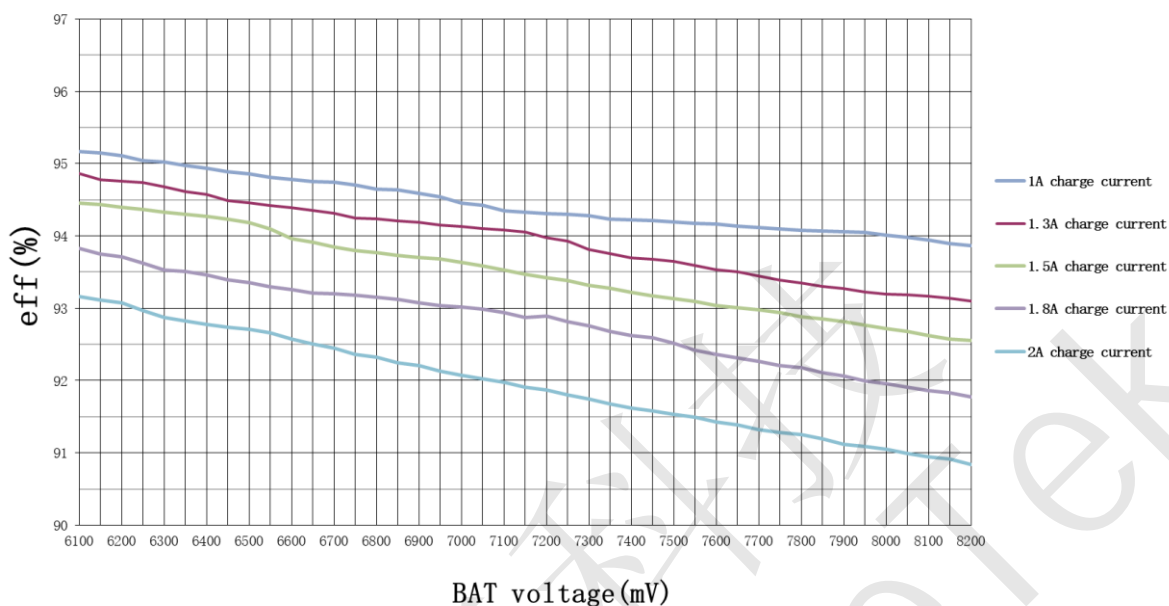
IP2326-2 series charging efficiency curve VIN=5V
