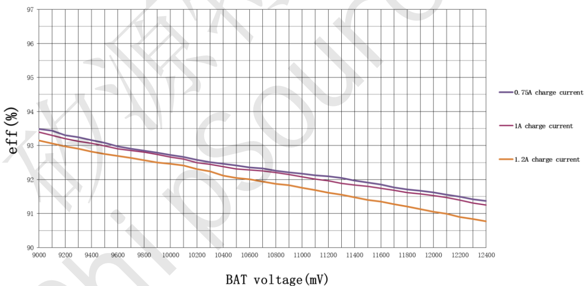
IP2326-3 series charging efficiency curve VIN=5V
