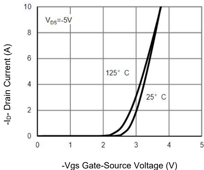
Figure 7 Transfer Characteristics
