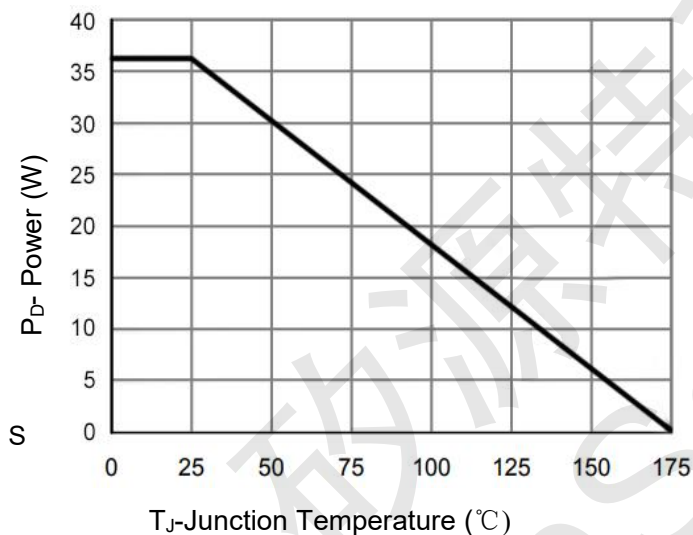
Figure 3 Power De-rating
