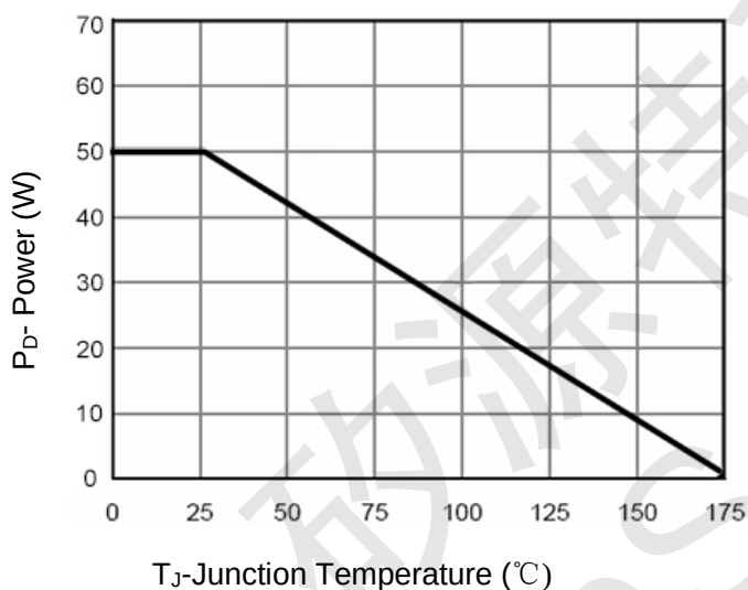
Figure 3 Power De-rating
