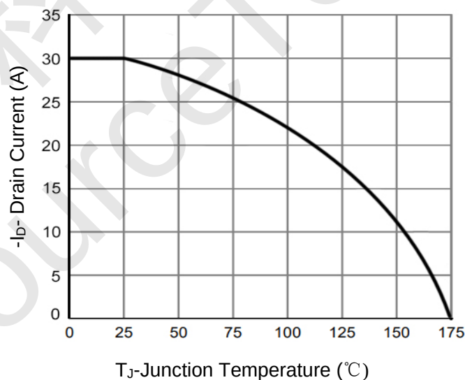
Figure 4 Drain Current
