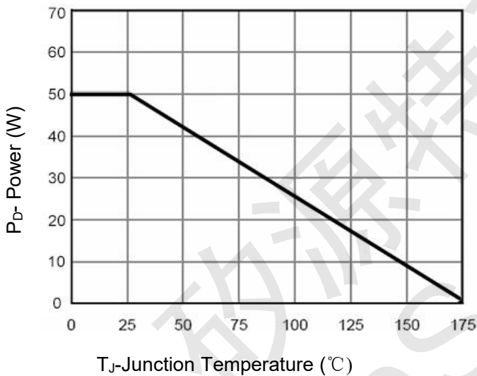
Figure 3 Power De-rating
