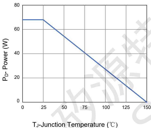
Figure 3 Power De-rating
