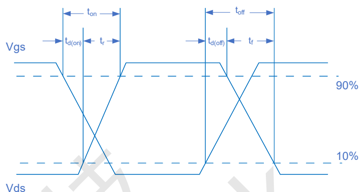
Figure 2 Switching Waveform
