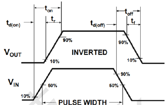
Figure 2 Switching Waveform
