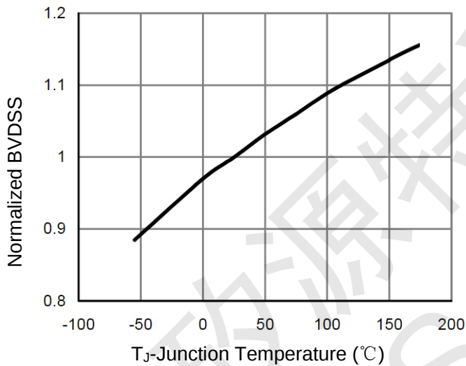
Figure 9 B_{VDS} vs T_J
