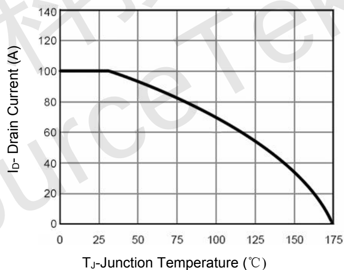
Figure 4 Drain Current
