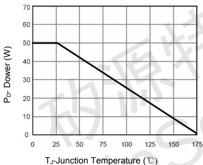
Figure 3 Power De-rating
