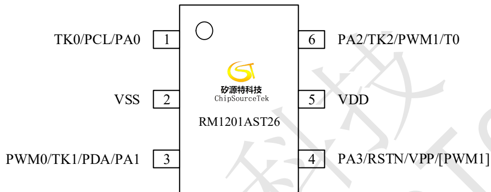
RM1201AST26 (SOT23-6)
