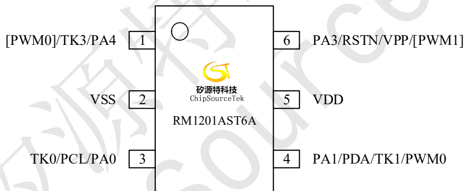
RM1201AST6A (SOT23-6)
