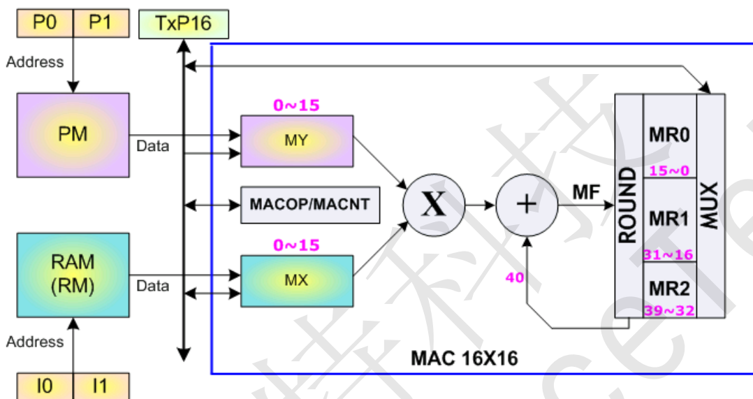
Figure 5.5 MAC Architecture
