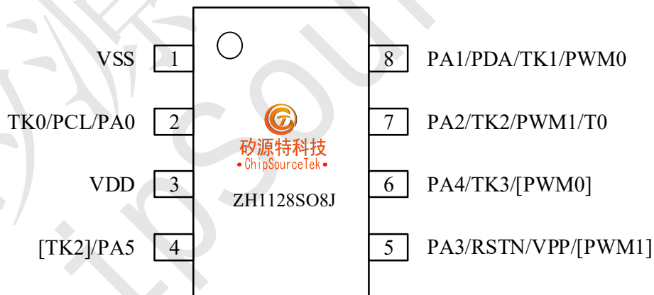
ZH1128SO8J (SOP8)
