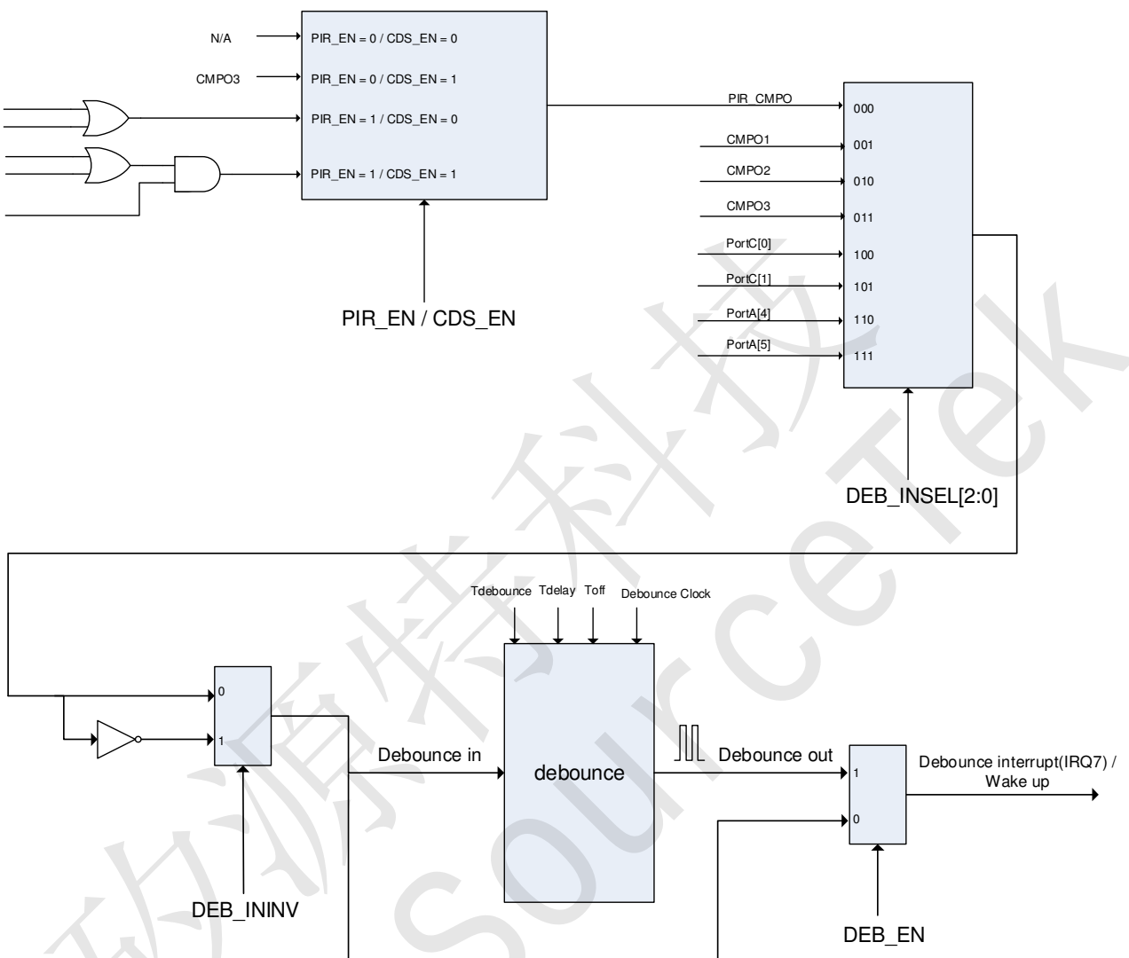
Figure 7.8 De-bounce Input Source
