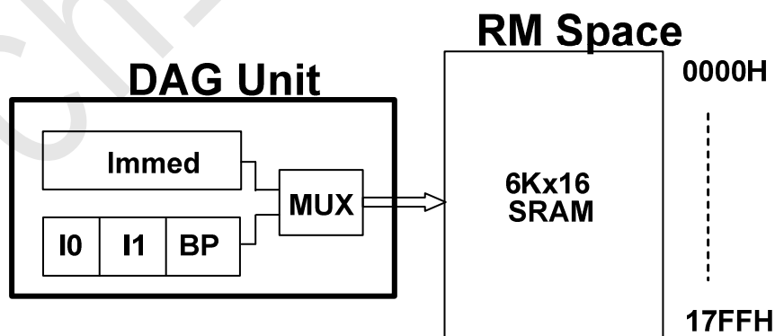
Figure 6.3 RM block diagram
