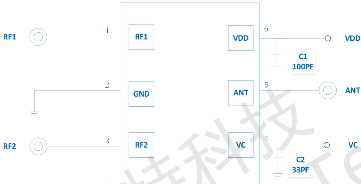
Figure 2 Application Schematic
