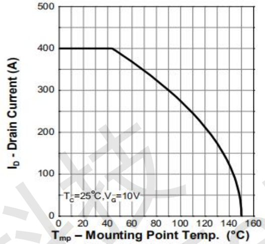
Figure 2. Current Capability
