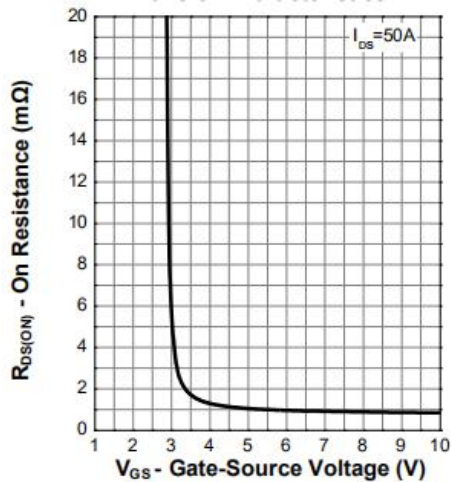
Figure 7. Transfer Characteristics
