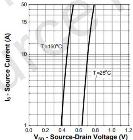
Figure 10. Diode Forward Current
