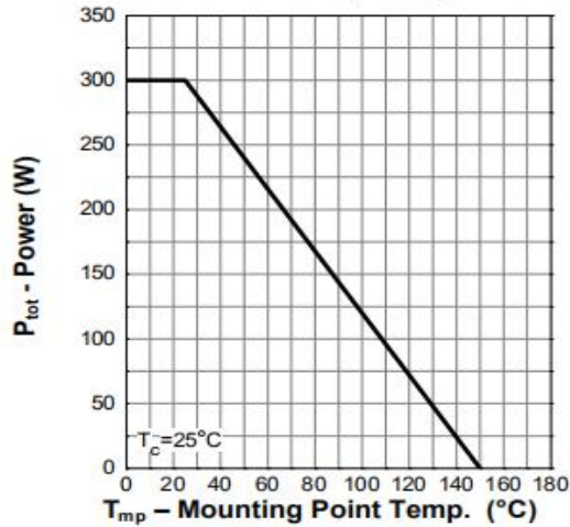
Figure 1. Power Capability
