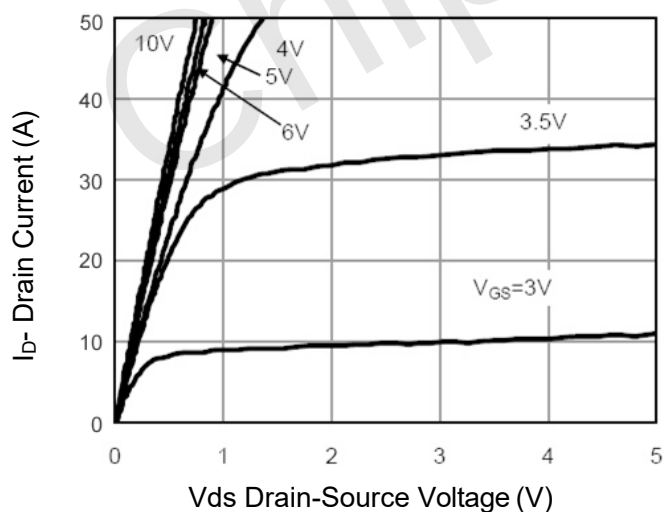
Figure 5 Output Characteristics
