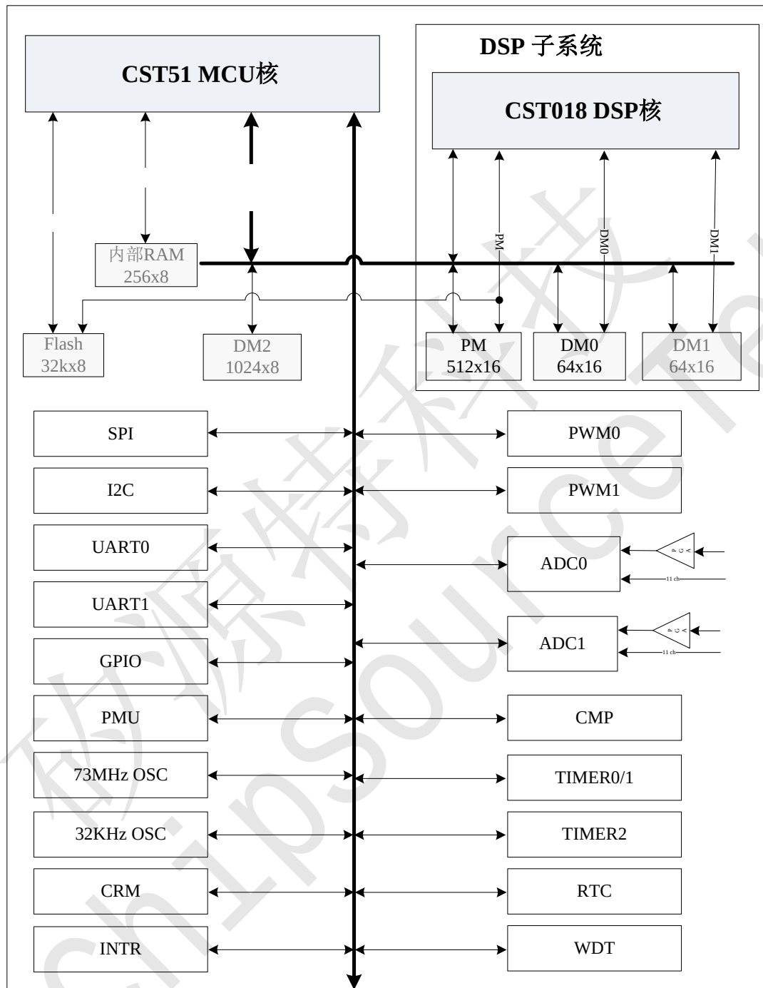
Figure 1 CST1808R 结构框图
