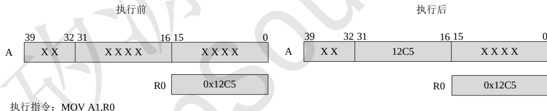
Figure 31 MOV A1,Rn 指令
