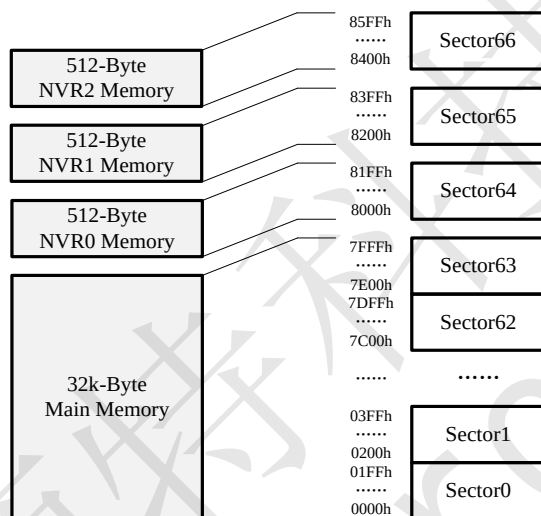
Figure 56 FLASH Memory
