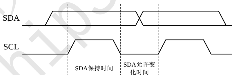
Figure 137 I2C 位传输
