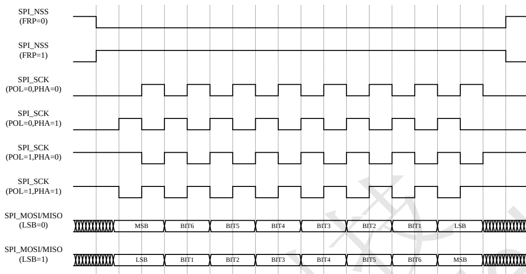
Figure 156 SPI 时序
