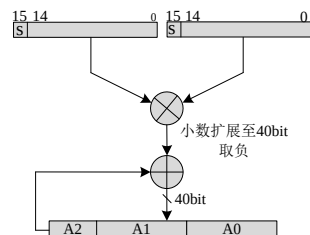
Figure 43 有符号小数乘减
