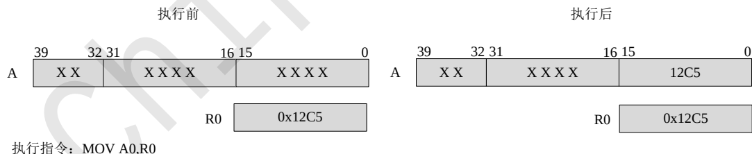
Figure 32 MOV A0,Rn 指令
