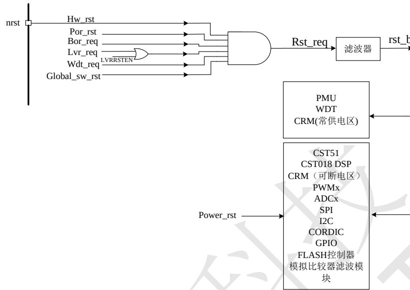
Figure 11 CST1808R 复位
