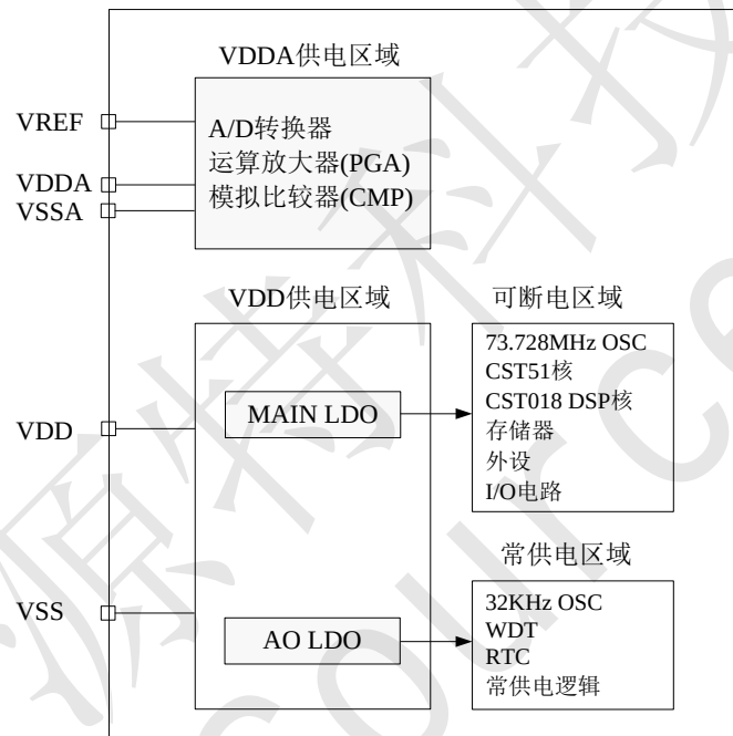
Figure 7 CST1808R 芯片供电示意图
