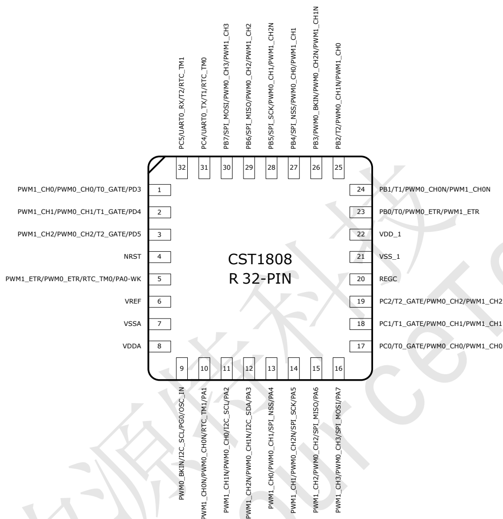
Figure 5 CST1808R 芯片 QFN32L 封装
