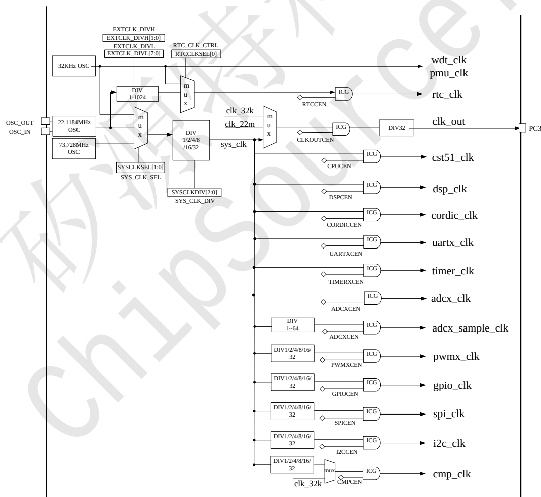
Figure 9 CST1808R 时钟树
