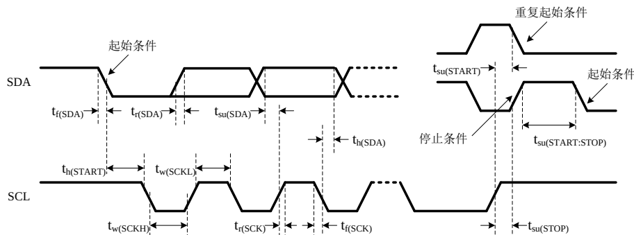
Figure 208 I2C 总线波形示意图
