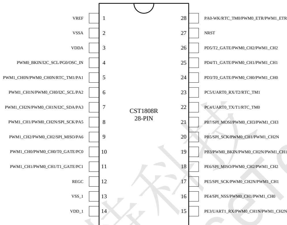
Figure 6 CST1808R 芯片 TSSOP28L 封装
